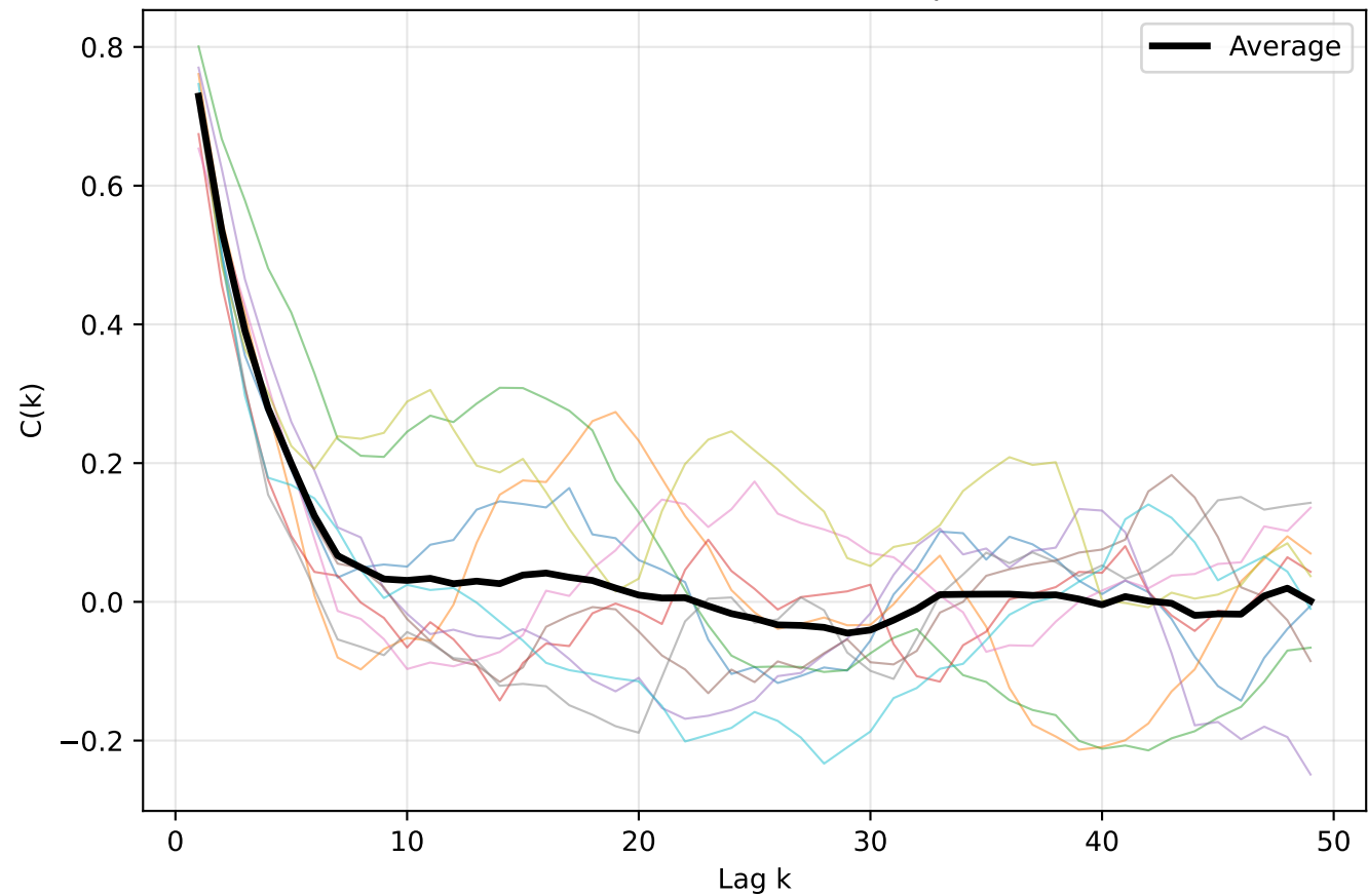
LUMO - All autocorrelation for Experiment 1
