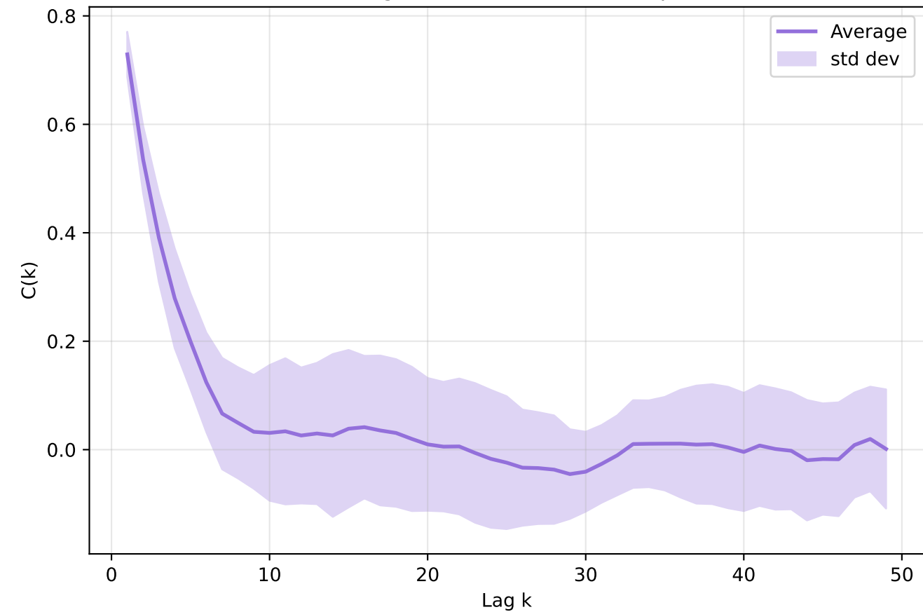
LUMO - Average autocorrelation for Experiment 1
