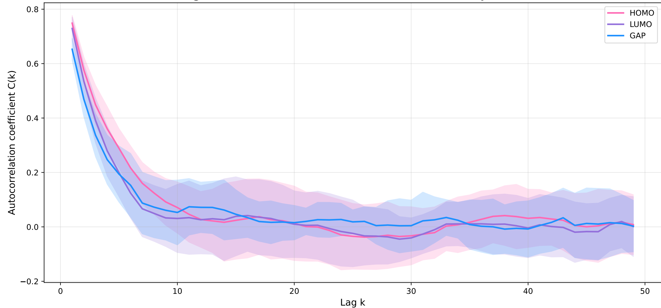
Average autocorrelations (HOMO, LUMO, GAP) for Experiment 1
