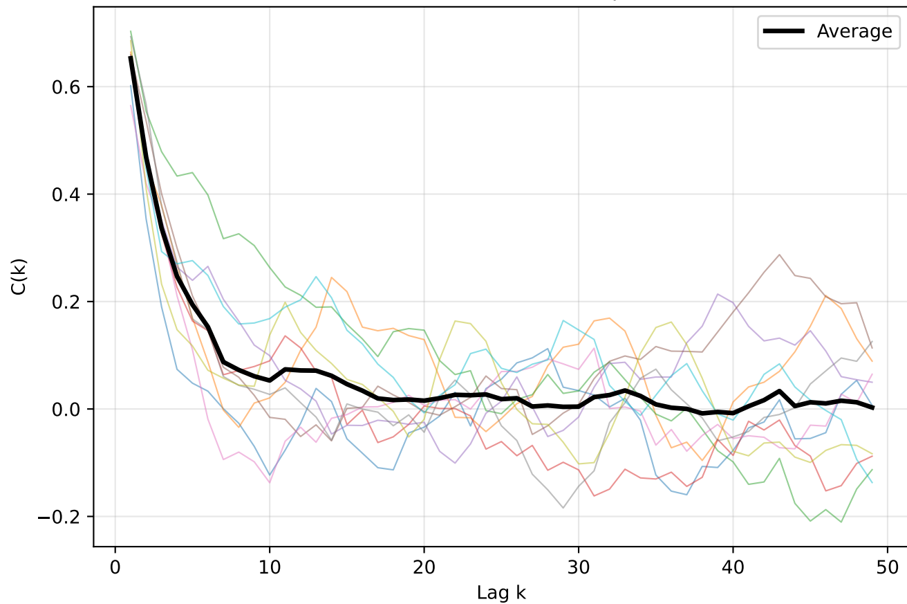
GAP - All autocorrelation for Experiment 1
