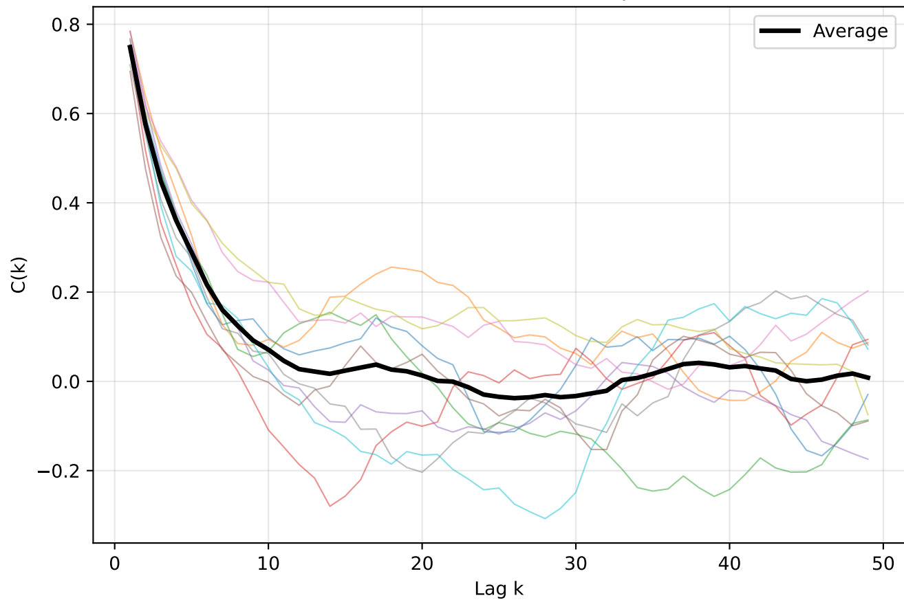
HOMO - All autocorrelation for Experiment 1
