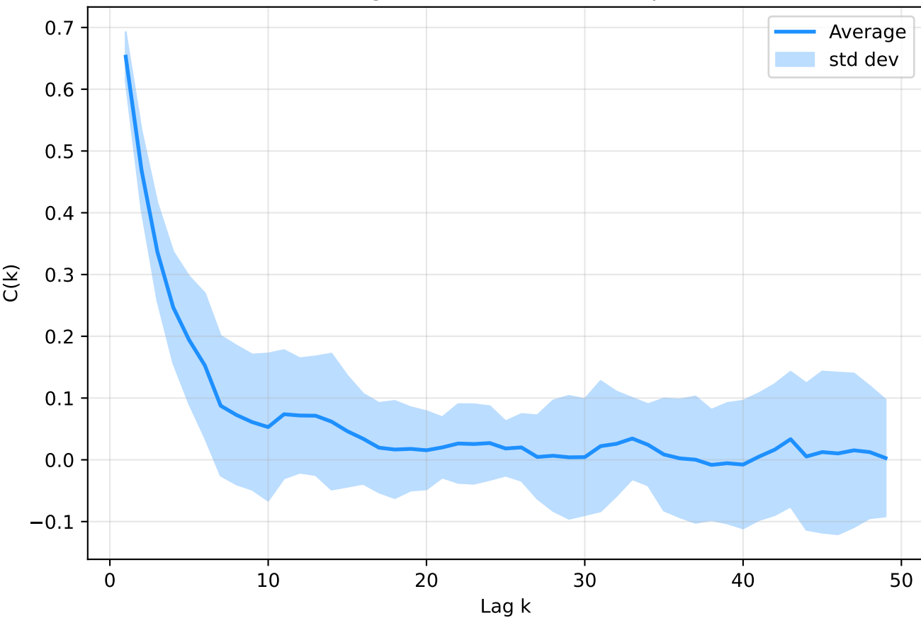
GAP - Average autocorrelation for Experiment 1
