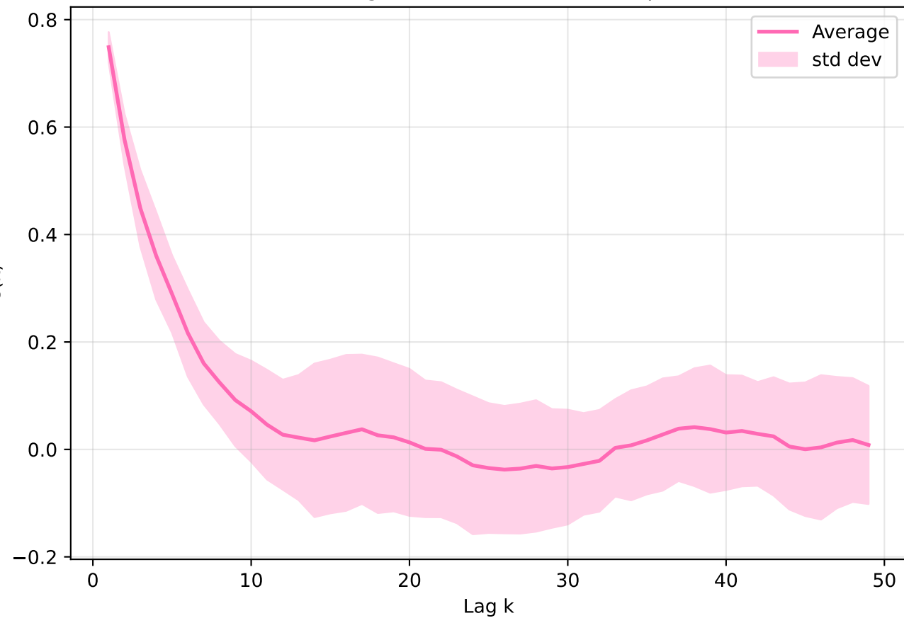
HOMO - Average autocorrelation for Experiment 1
